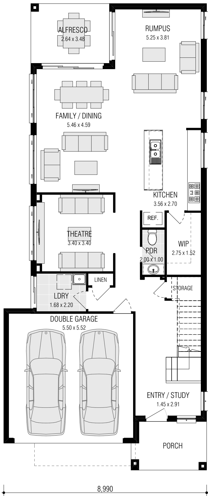
GROUND FLOOR
