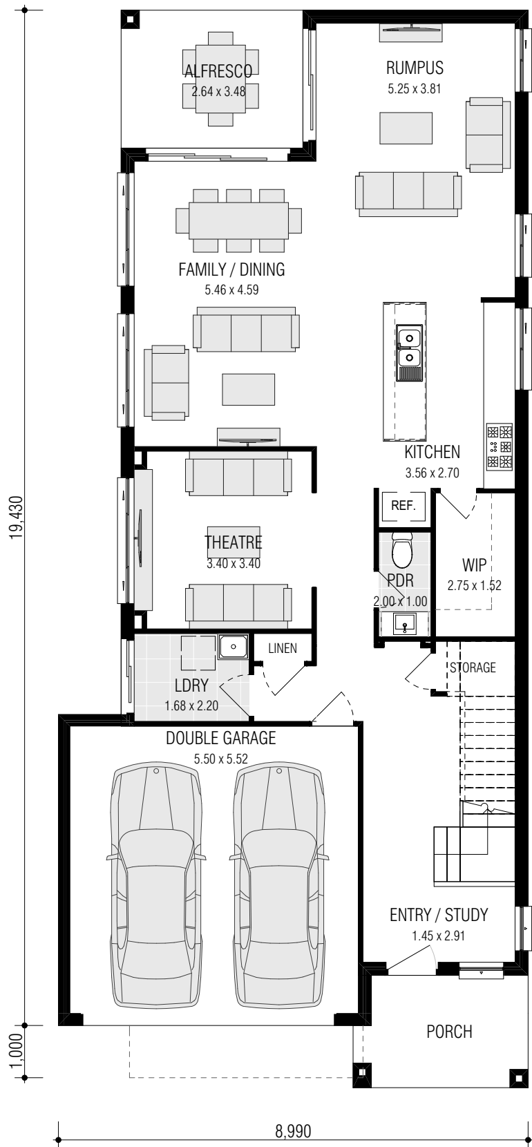
GROUND FLOOR
