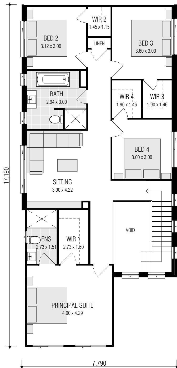
FIRST FLOOR
