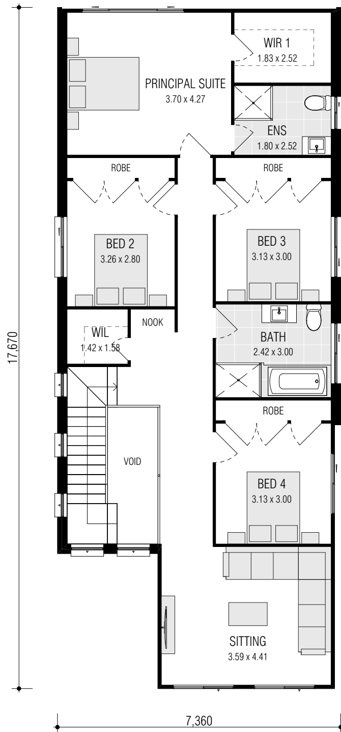
FIRST FLOOR
