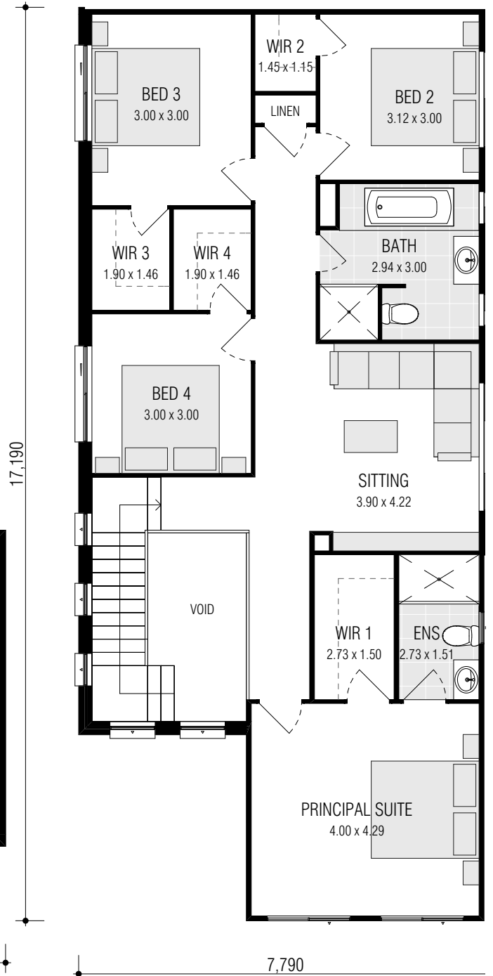
FIRST FLOOR
