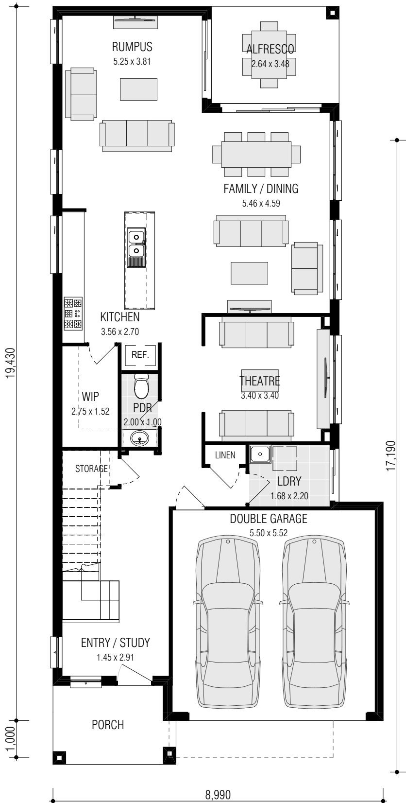
GROUND FLOOR
