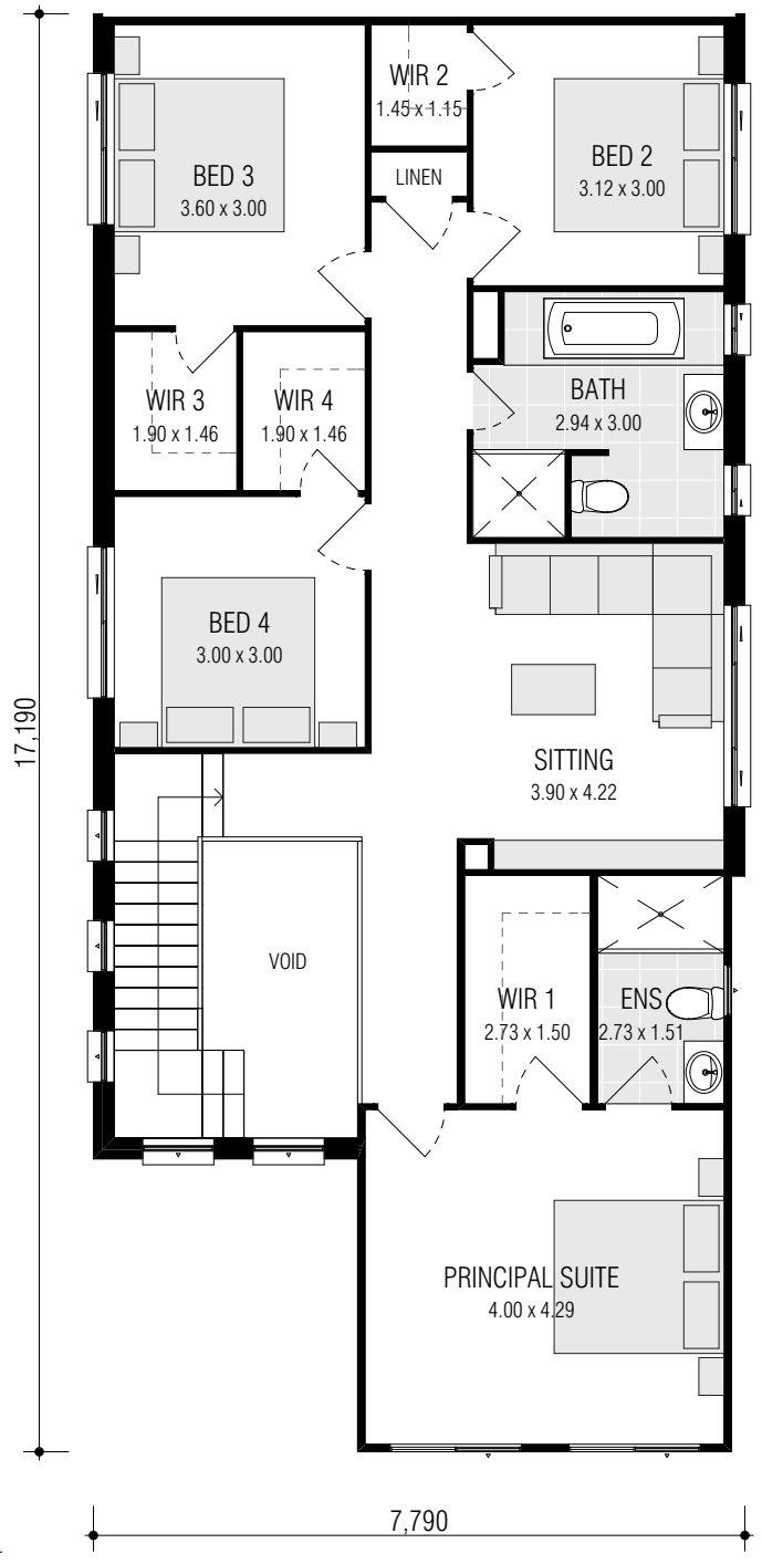
FIRST FLOOR
