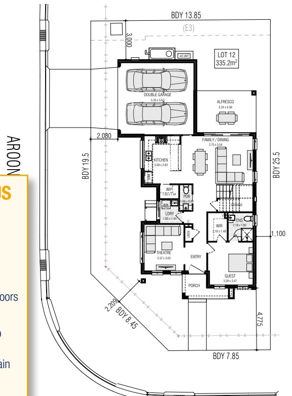
(E3) PROPOSED EASEMENT TO DRAIN WATER 1.2 & 1.5 WIDE
